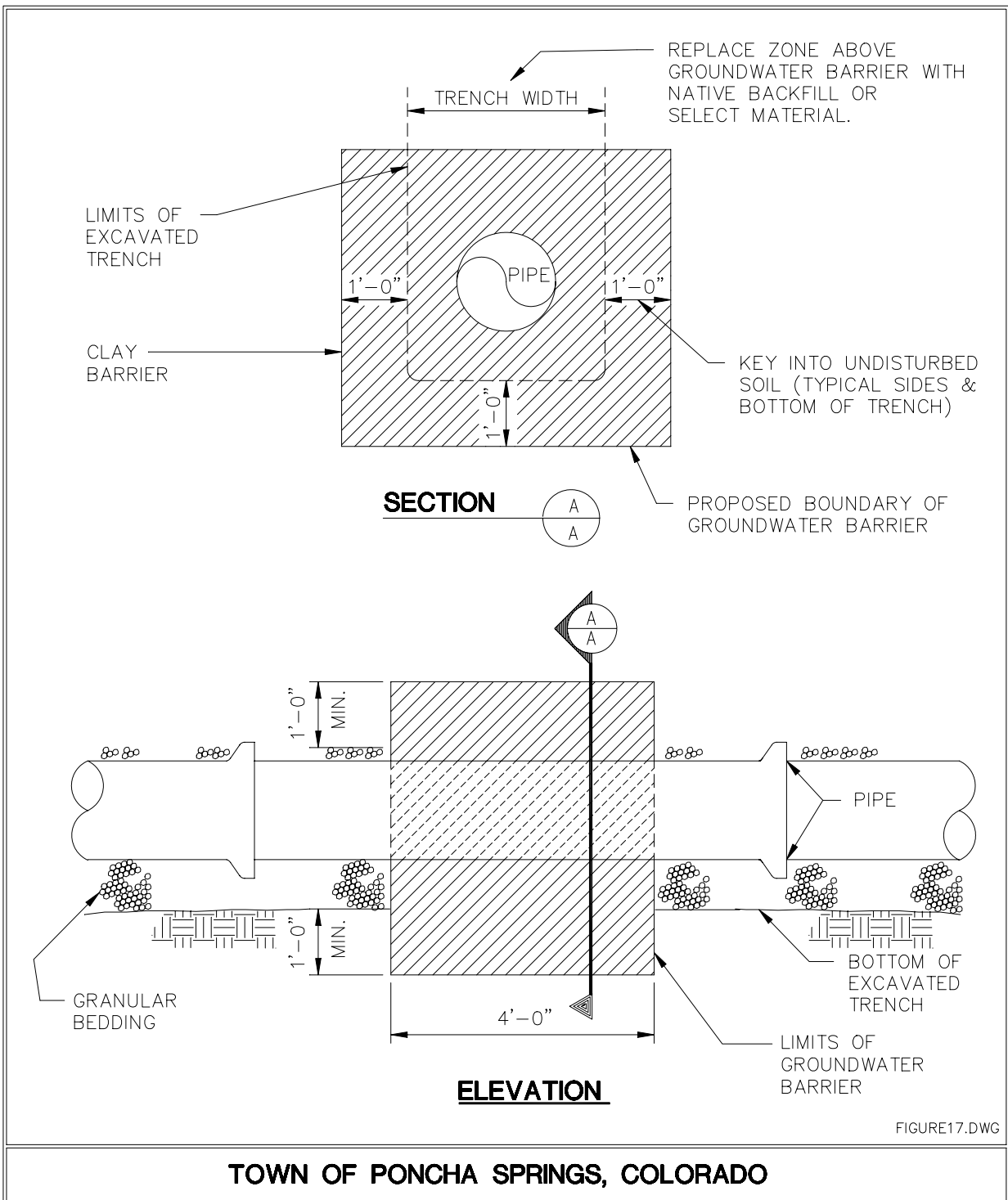
FIGURE 17 GROUNDWATER BARRIER DETAIL
