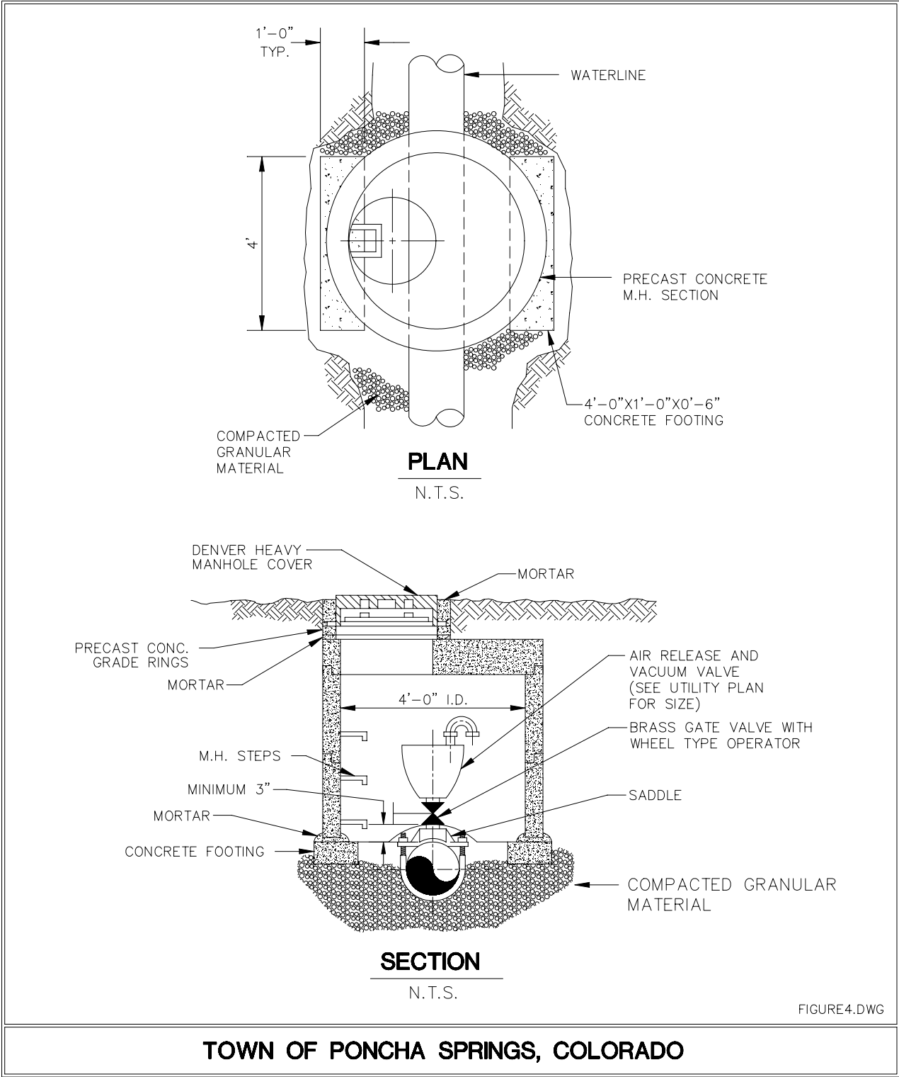
FIGURE 4 STANDARD AIR AND VACUUM RELIEF VALVE INSTALLATION
